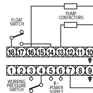
Connections with pressure switch and 1 float switch
